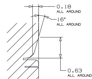
CAMERA CONTROL CHAMFER
