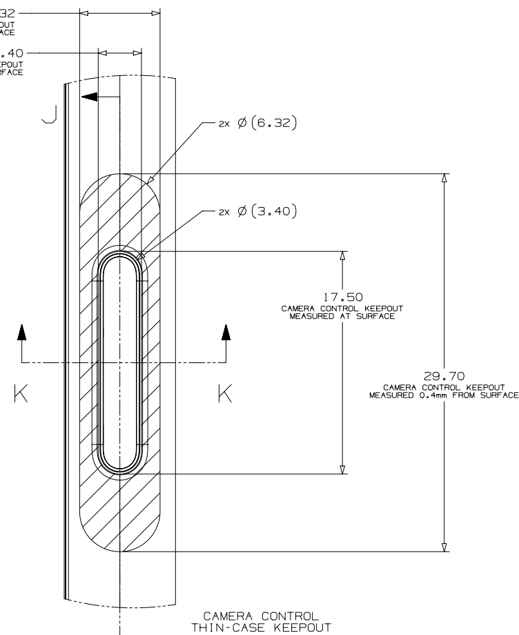
DETAIL E
