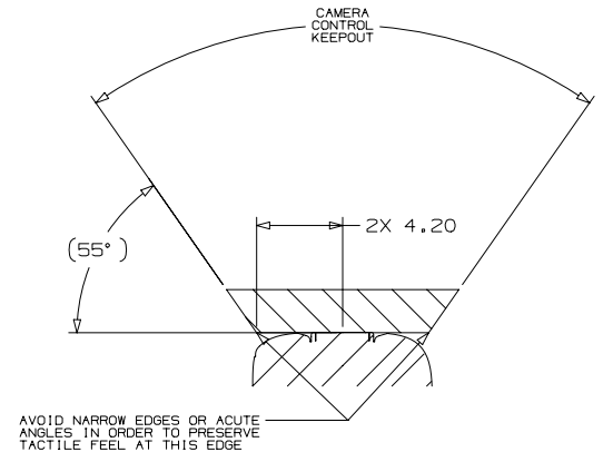
CAMERA CONTROL TYPICAL KEEPOUT
