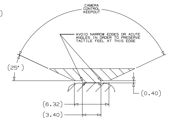
CAMERA CONTROL THIN-CASE KEEPOUT
