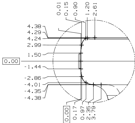
PROFILE (ALL SIDES) DETAIL B
